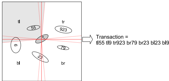
Fig. 1. Creating transaction from a neighborhood. The area around a central visual word v_c is divided into sections. Each section is labeled ( tl\dots ) and the label is appended to the visual word ids.
